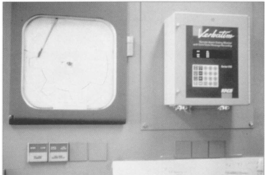
RACO Verbatim autodialer is mounted inside the Hampton Water Works control center for easy access. Because the unit is designed for operation in harsh environments, it can also be placed outdoors. Because of its low cost and simplicity of operation, the Verbatim unit is suited for use in smaller water distribution systems. (Photo by John Rock)
